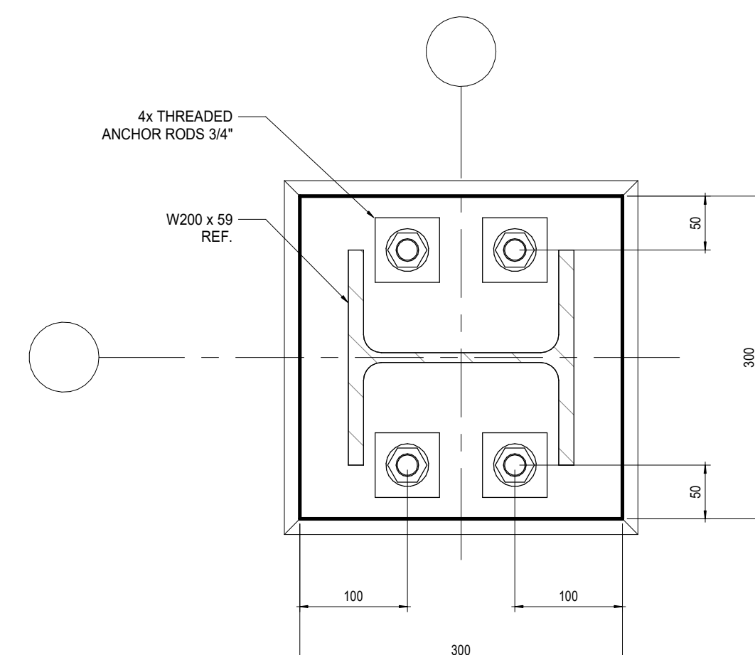
BASE PLATE DETAIL 4-1 1 : 5
