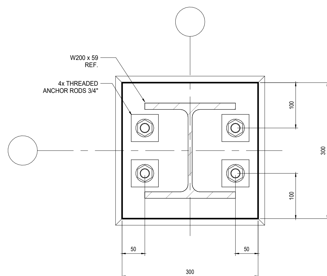
BASE PLATE DETAIL 3-1 1 : 5
